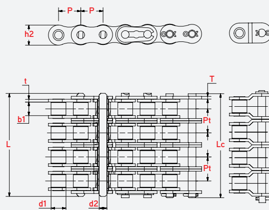
Quadruple Strand
