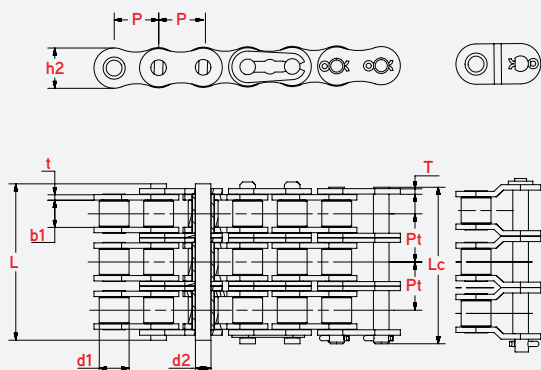
Triple Strand
