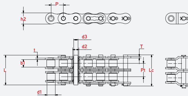
Double Strand
