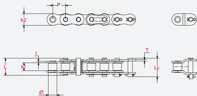
Simple Strand
