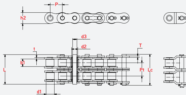
Double Strand
